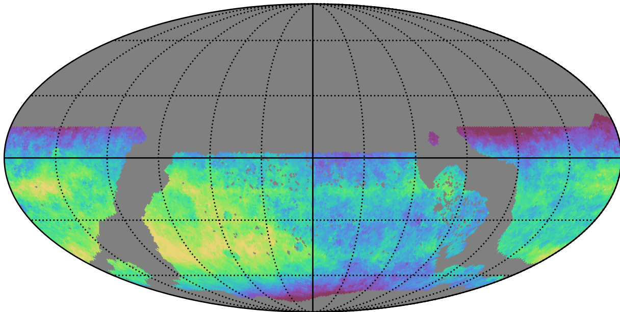
too_10_4v3.4_10yrs WFD z band: Median fiveSigmaDepth
