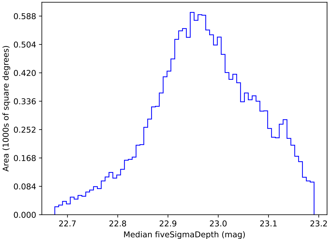
too_10_4v3.4_10yrs WFD z band: Median fiveSigmaDepth
