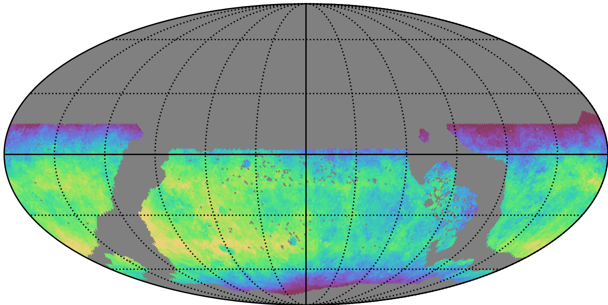
too_10_4v3.4_10yrs WFD y band: Median fiveSigmaDepth
