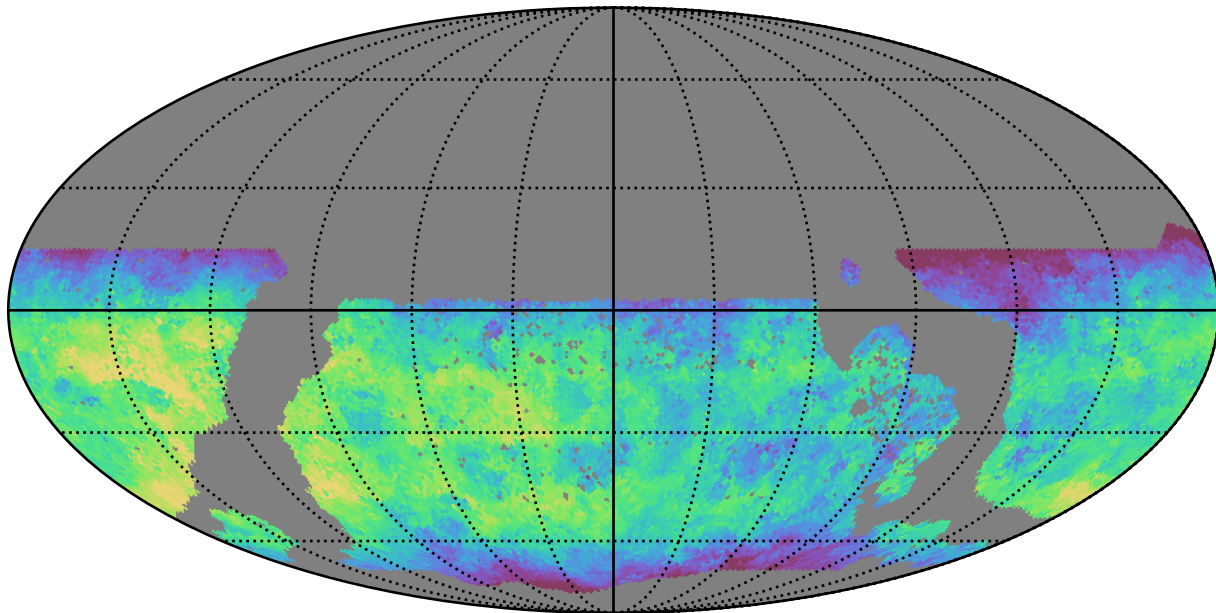
too_10_4v3.4_10yrs WFD u band: Median fiveSigmaDepth
