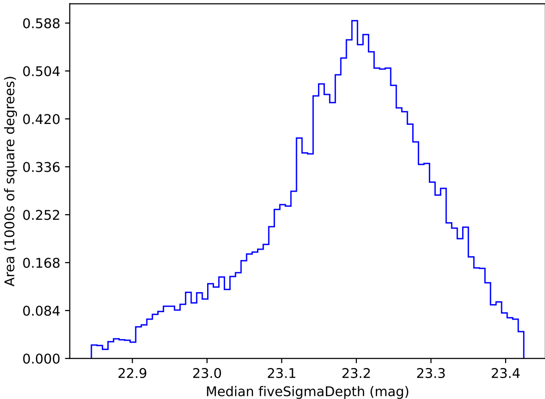
too_10_4v3.4_10yrs WFD u band: Median fiveSigmaDepth
