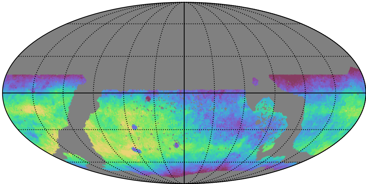
too_10_4v3.4_10yrs WFD r band: Median fiveSigmaDepth
