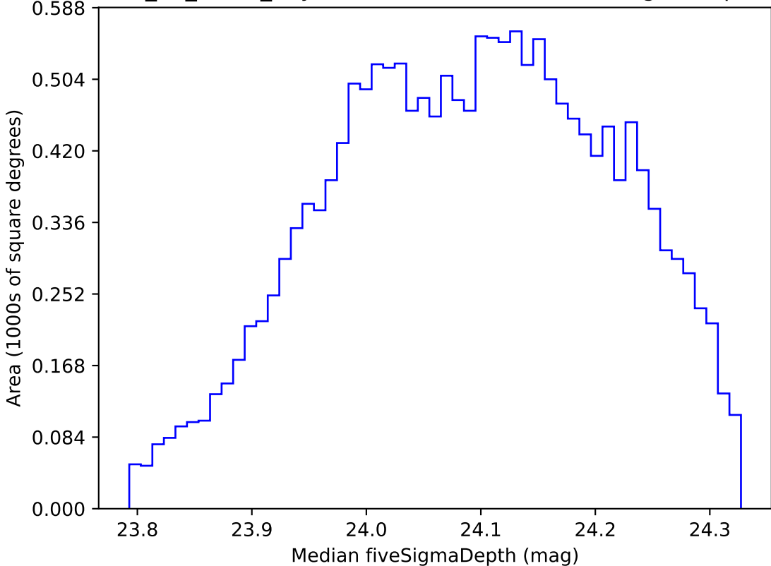
too_10_4v3.4_10yrs WFD r band: Median fiveSigmaDepth
