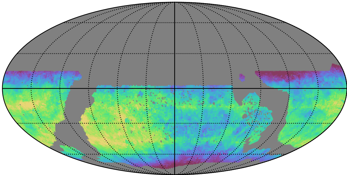
too_10_4v3.4_10yrs WFD i band: Median fiveSigmaDepth
