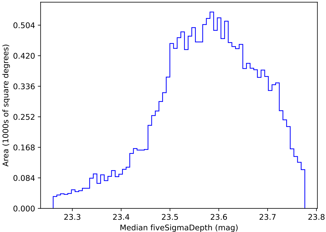
too_10_4v3.4_10yrs WFD i band: Median fiveSigmaDepth
