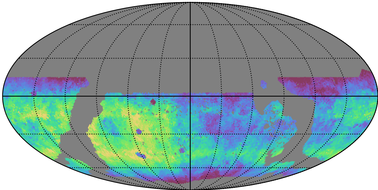
too_10_4v3.4_10yrs WFD g band: Median fiveSigmaDepth
