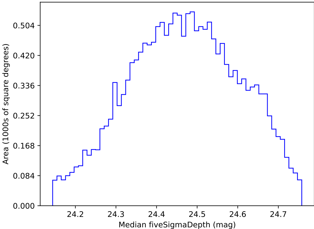
too_10_4v3.4_10yrs WFD g band: Median fiveSigmaDepth
