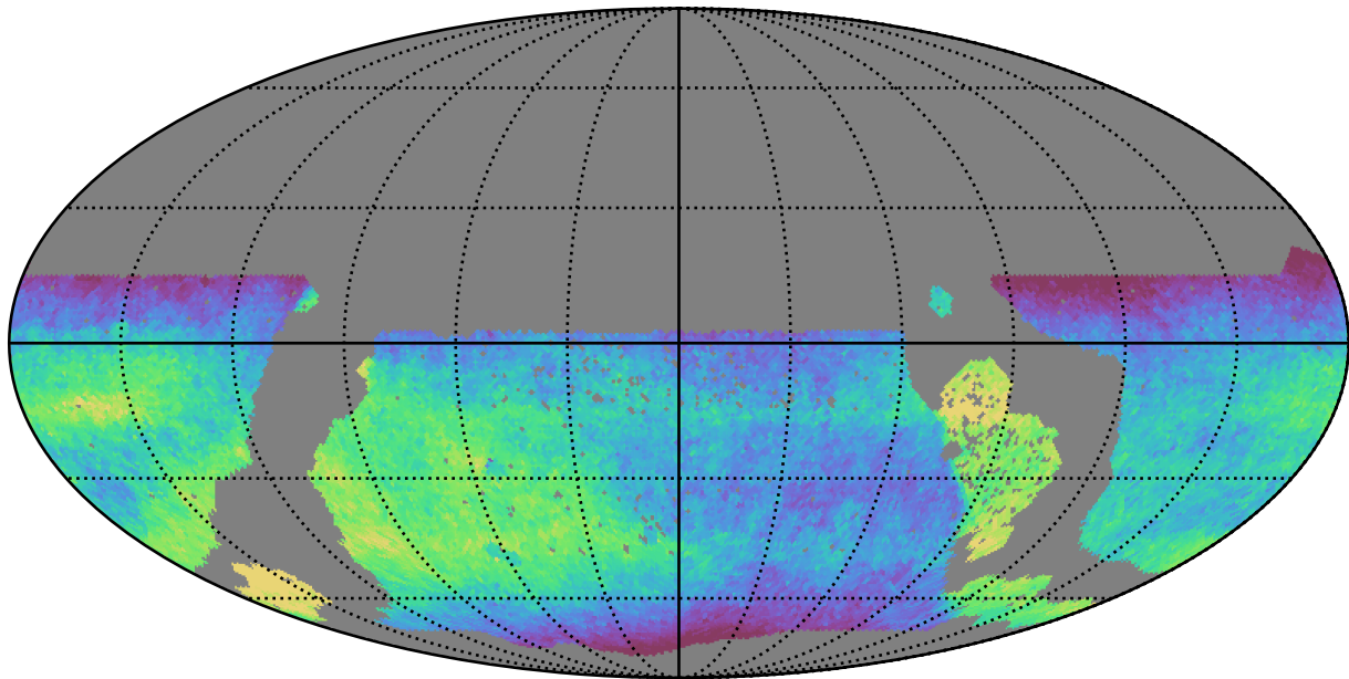
too_10_4v3.4_10yrs WFD all bands: Median fiveSigmaDepth
