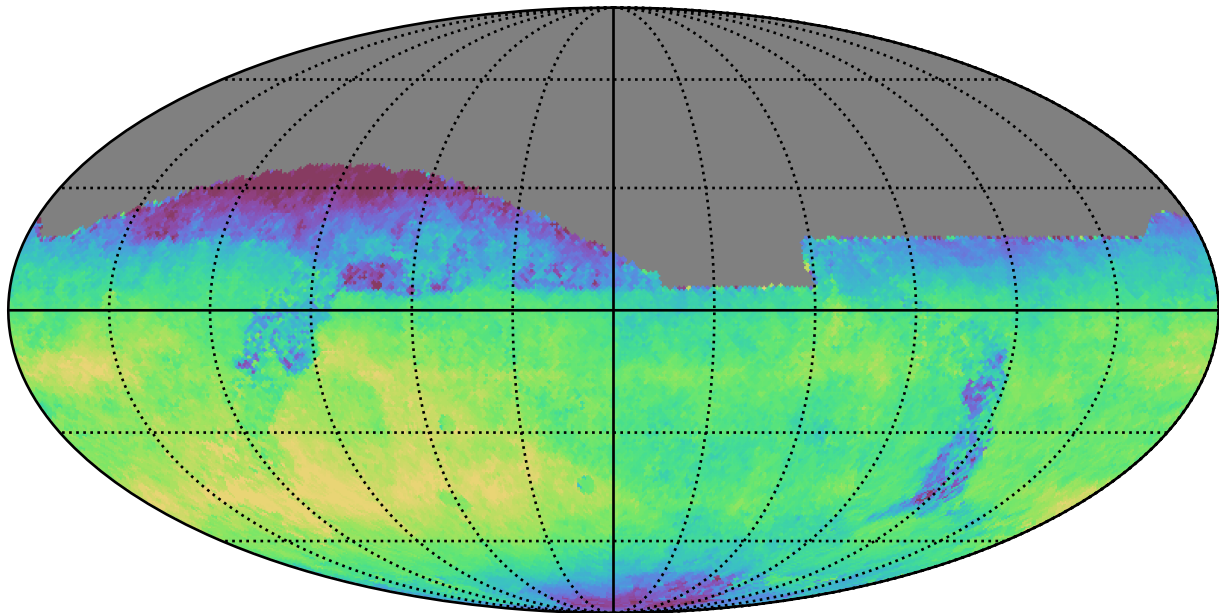
too_10_4v3.4_10yrs All sky z band: Median fiveSigmaDepth
