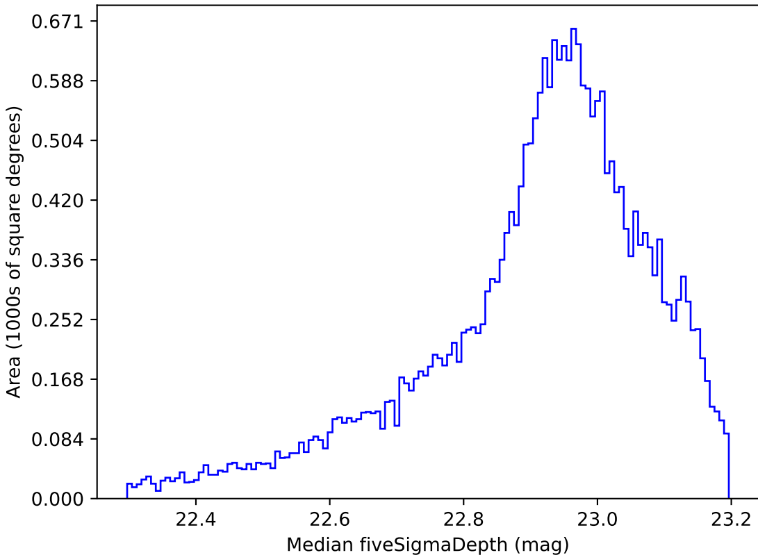
too_10_4v3.4_10yrs All sky z band: Median fiveSigmaDepth
