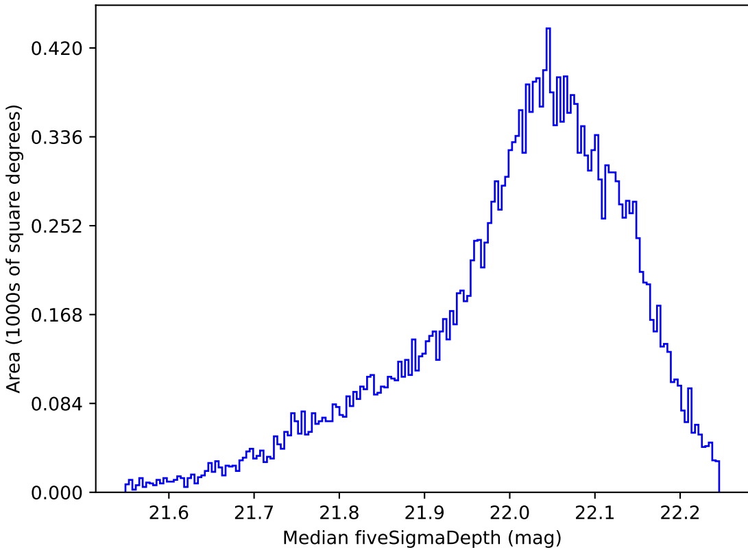
too_10_4v3.4_10yrs All sky y band: Median fiveSigmaDepth
