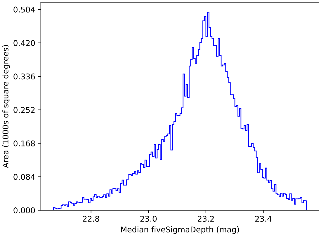
too_10_4v3.4_10yrs All sky u band: Median fiveSigmaDepth
