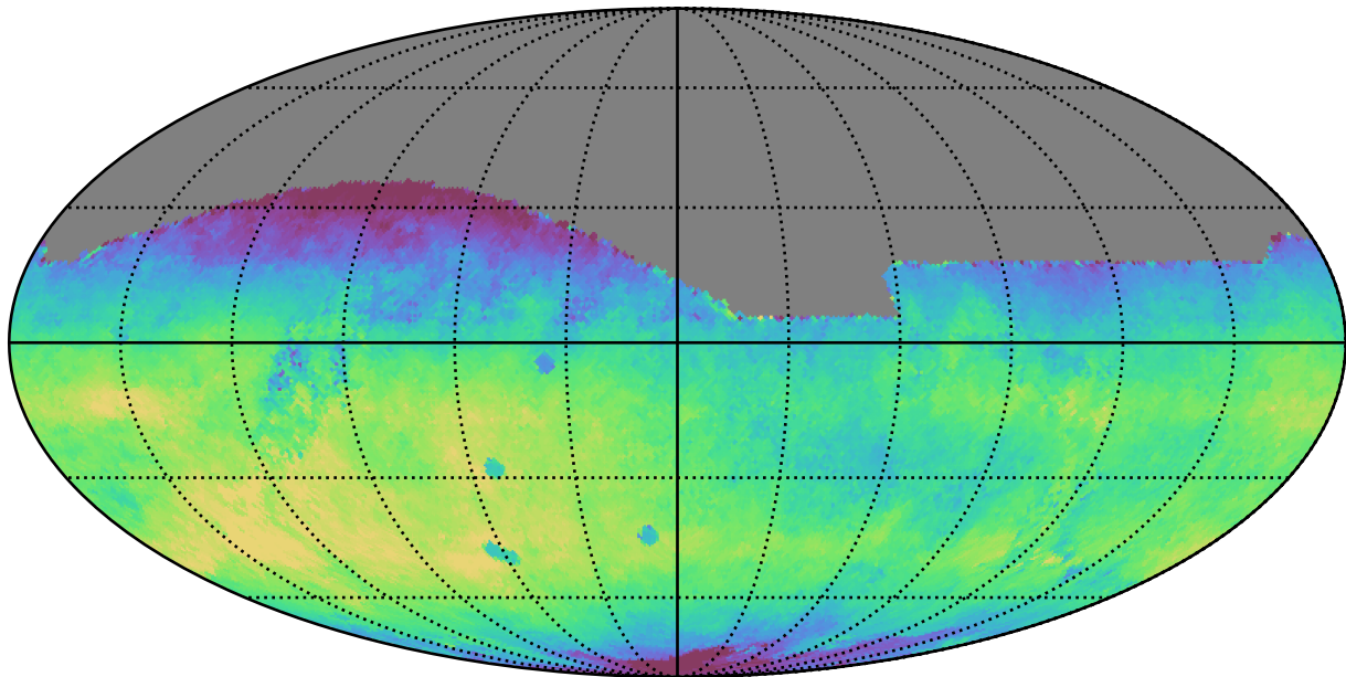
too_10_4v3.4_10yrs All sky r band: Median fiveSigmaDepth
