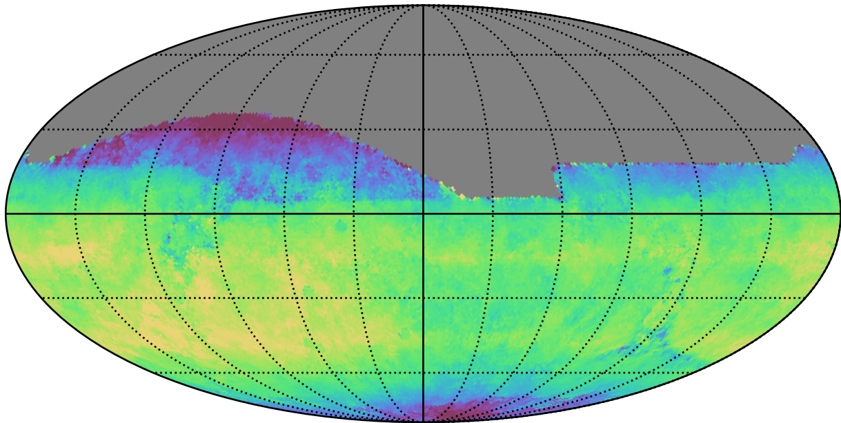
too_10_4v3.4_10yrs All sky i band: Median fiveSigmaDepth
