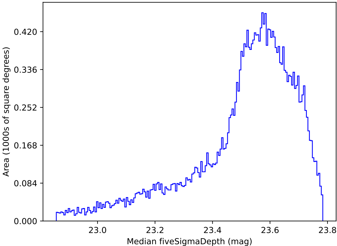
too_10_4v3.4_10yrs All sky i band: Median fiveSigmaDepth
