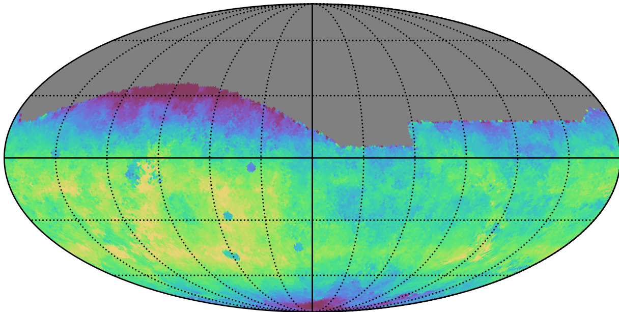
too_10_4v3.4_10yrs All sky g band: Median fiveSigmaDepth
