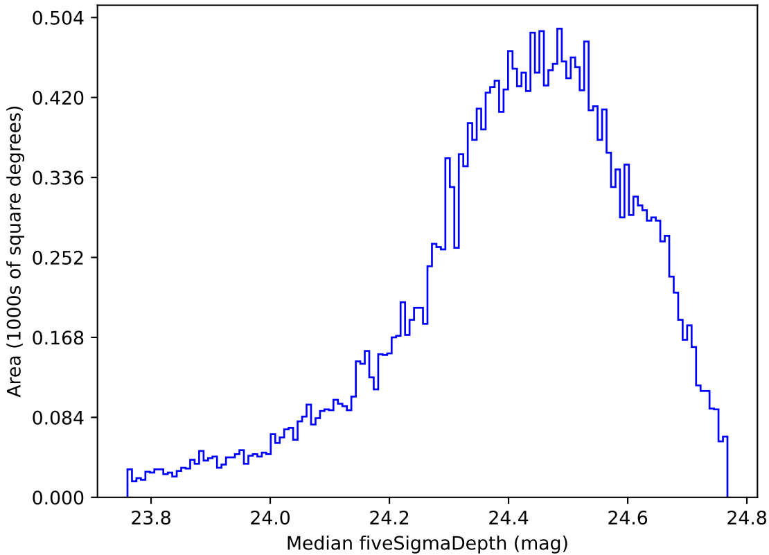
too_10_4v3.4_10yrs All sky g band: Median fiveSigmaDepth
