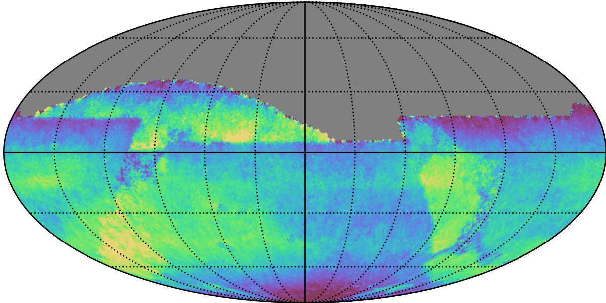
too_10_4v3.4_10yrs All sky all bands: Median fiveSigmaDepth
