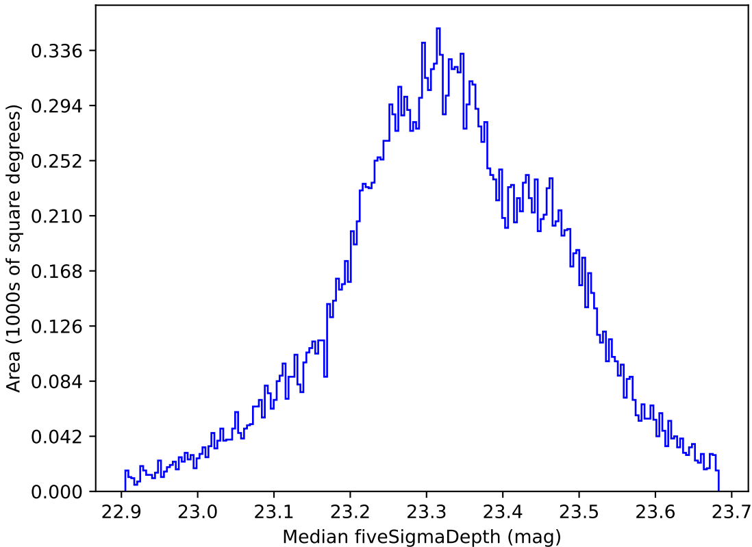
too_10_4v3.4_10yrs All sky all bands: Median fiveSigmaDepth
