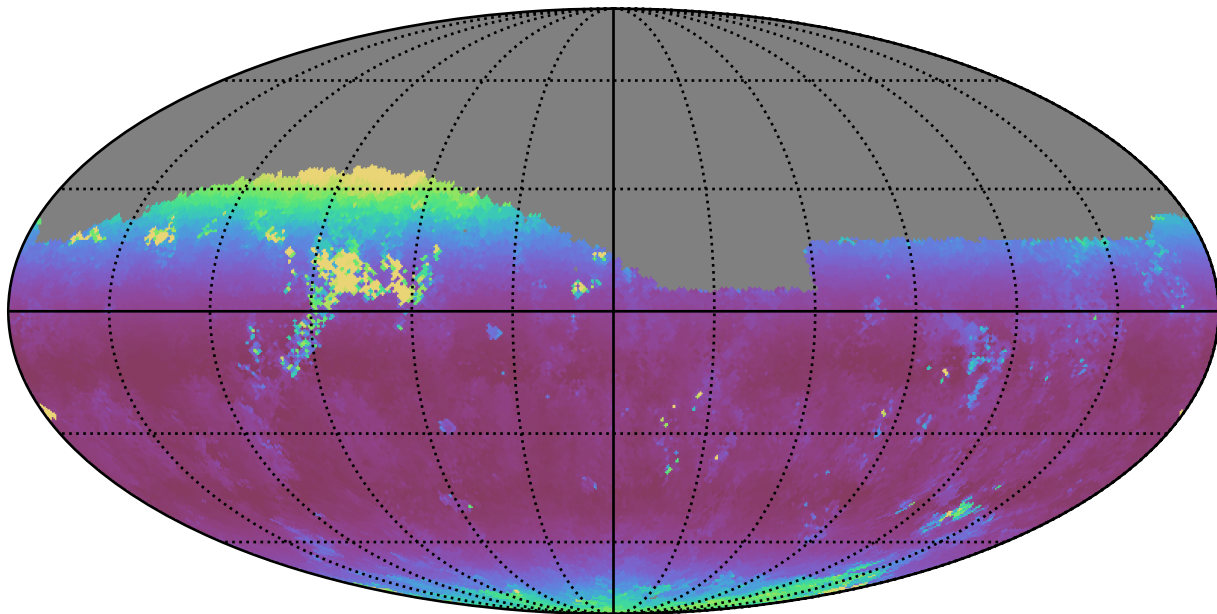
too_10_4v3.4_10yrs Yr 1 z band: Median airmass
