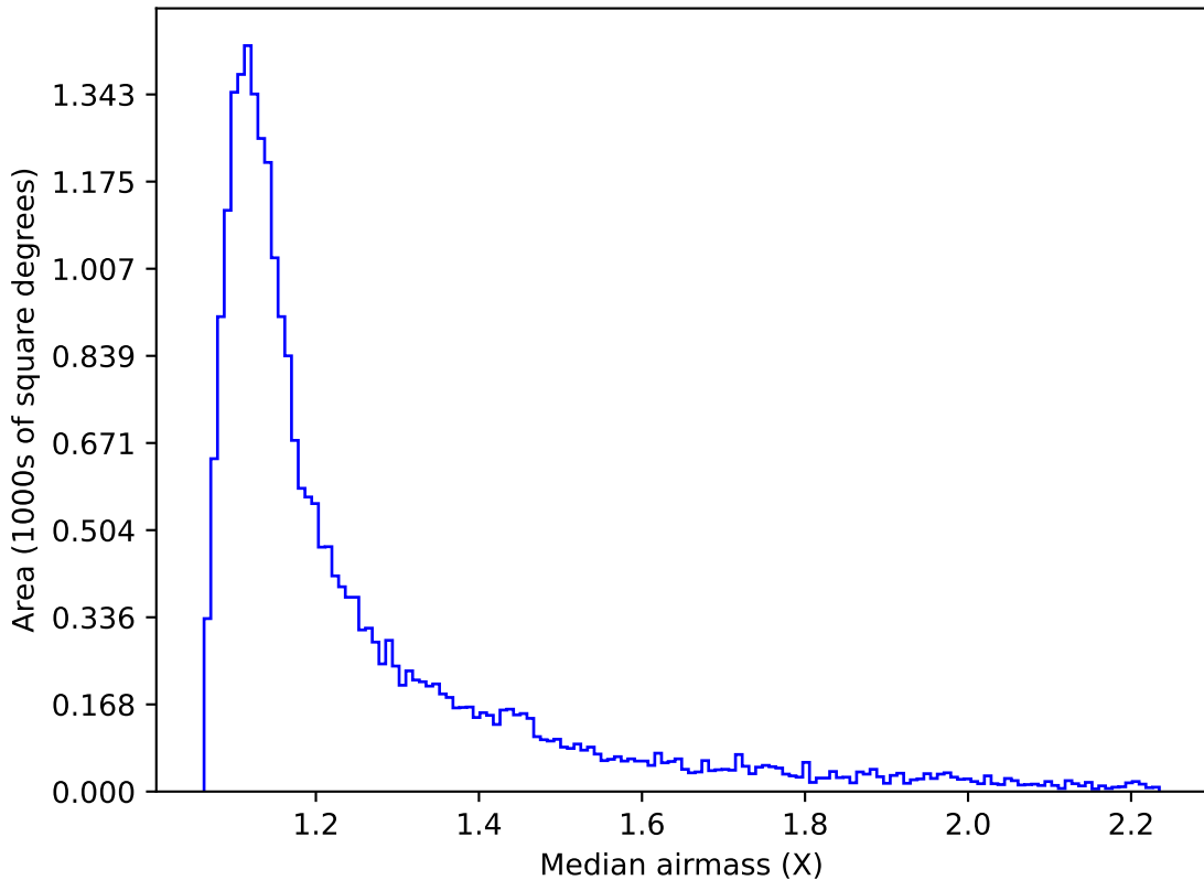
too_10_4v3.4_10yrs Yr 1 z band: Median airmass
