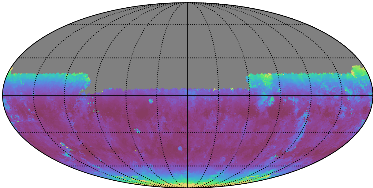
too_10_4v3.4_10yrs Yr 1 y band: Median airmass
