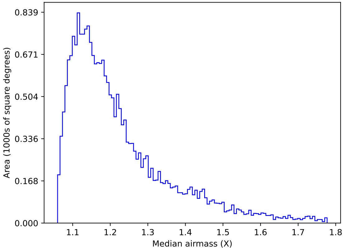
too_10_4v3.4_10yrs Yr 1 u band: Median airmass
