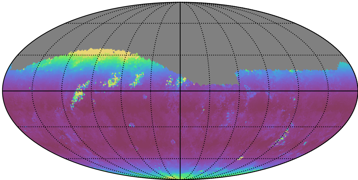
too_10_4v3.4_10yrs Yr 1 r band: Median airmass
