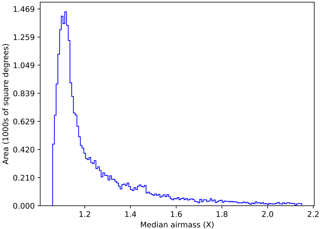
too_10_4v3.4_10yrs Yr 1 r band: Median airmass
