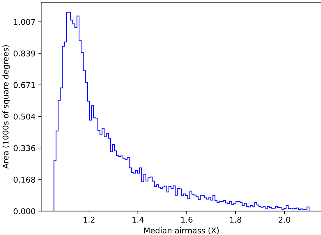
too_10_4v3.4_10yrs Yr 1 g band: Median airmass
