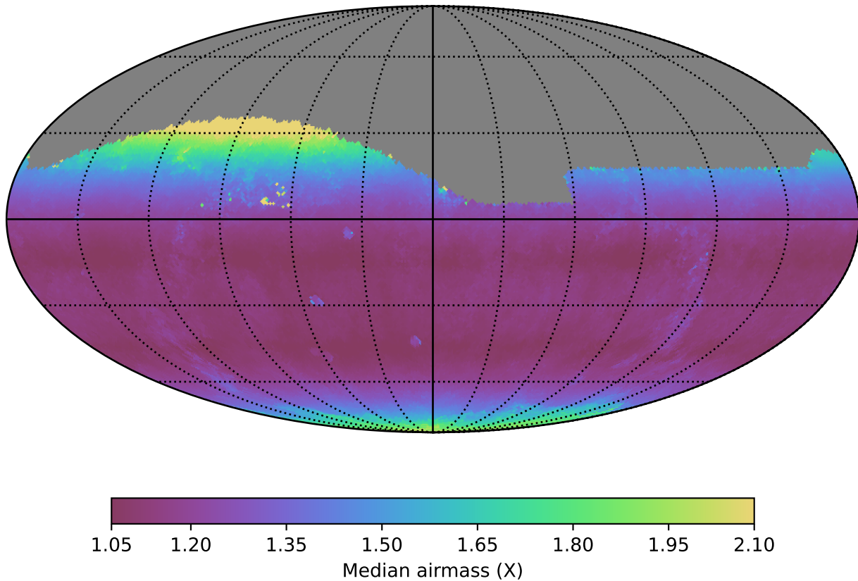
too_10_4v3.4_10yrs Yr 1 all bands: Median airmass
