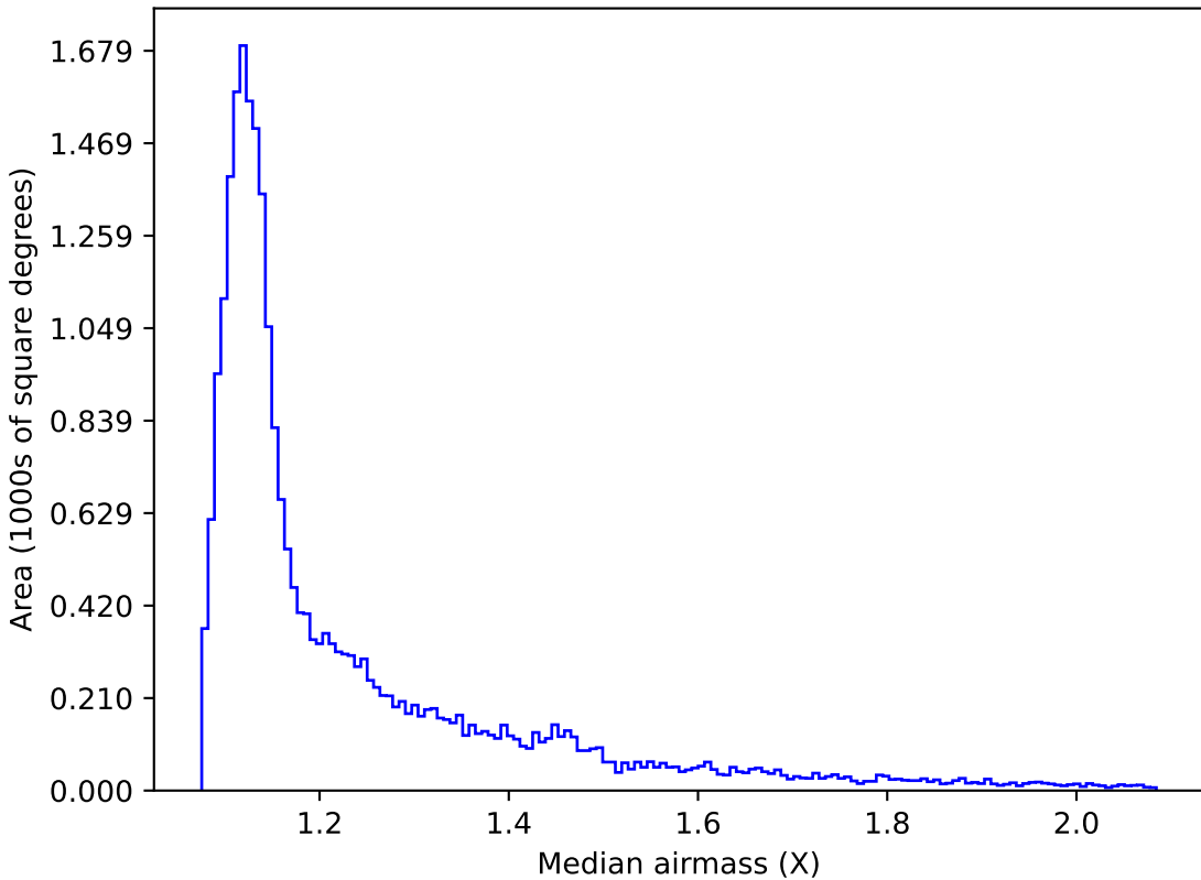
too_10_4v3.4_10yrs Yr 1 all bands: Median airmass
