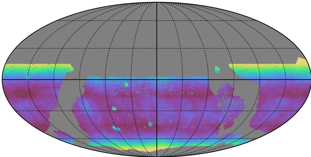
too_10_4v3.4_10yrs WFD z band: Median airmass
