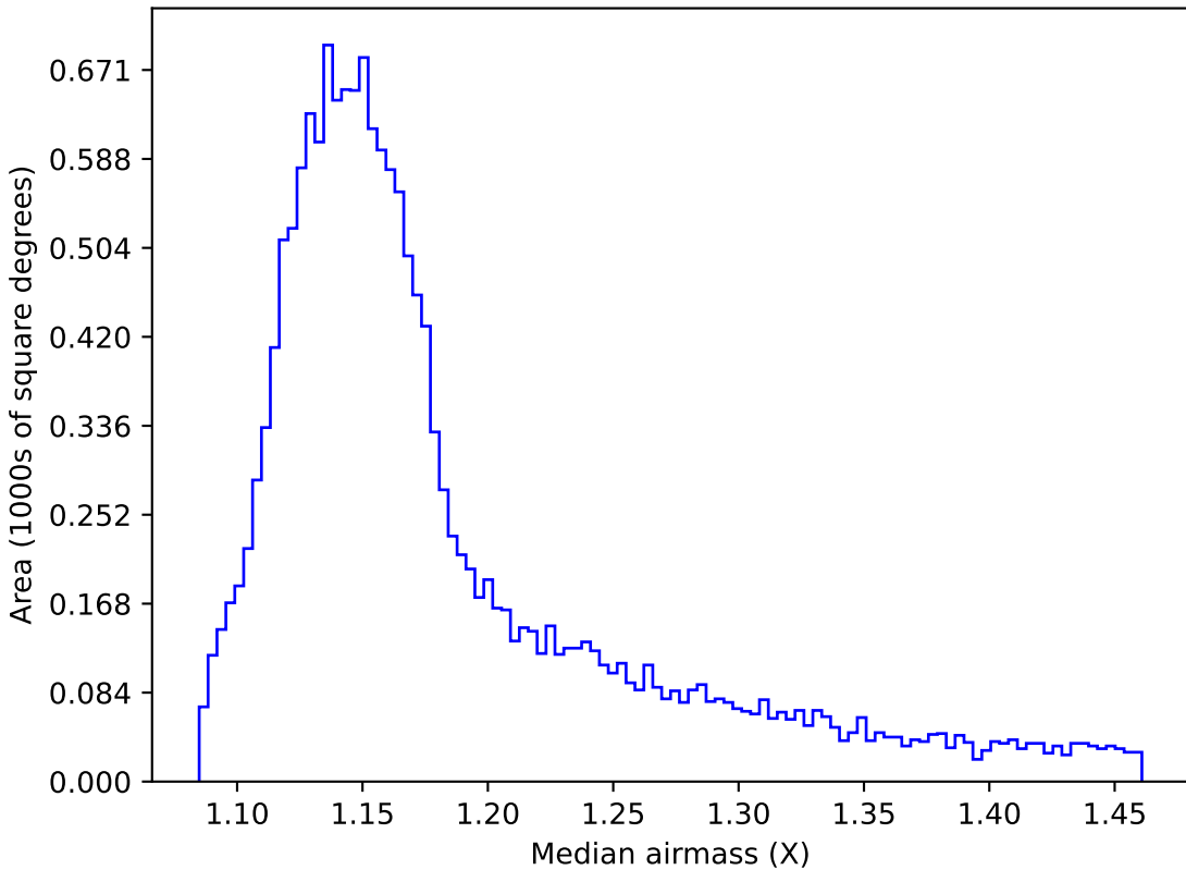
too_10_4v3.4_10yrs WFD z band: Median airmass
