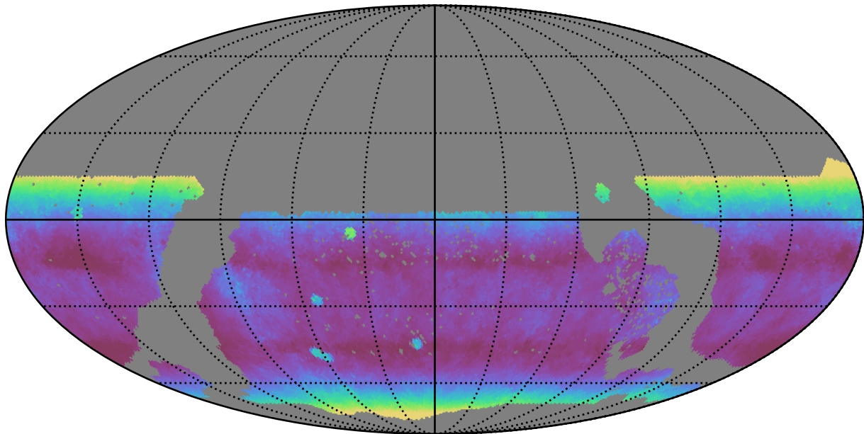
too_10_4v3.4_10yrs WFD y band: Median airmass
