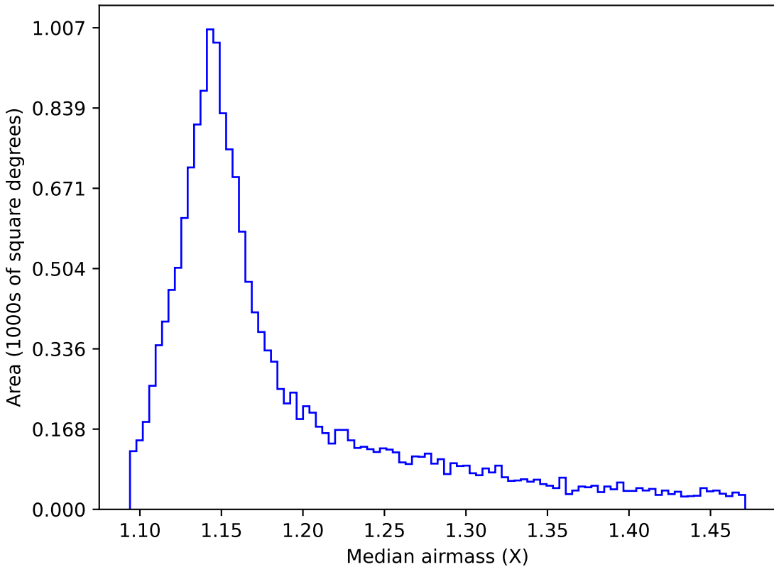
too_10_4v3.4_10yrs WFD y band: Median airmass
