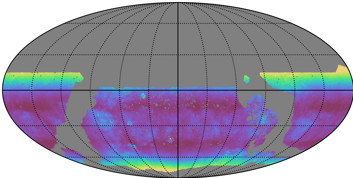
too_10_4v3.4_10yrs WFD u band: Median airmass
