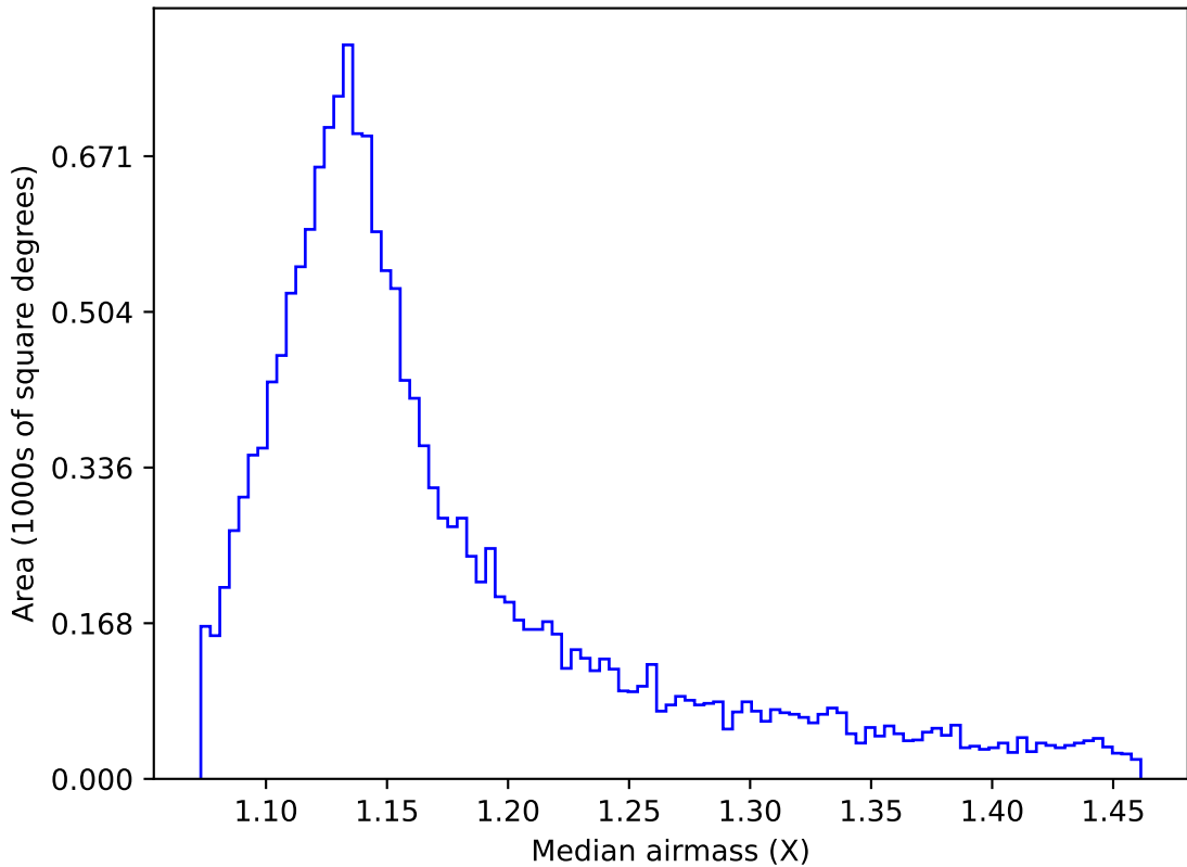
too_10_4v3.4_10yrs WFD u band: Median airmass
