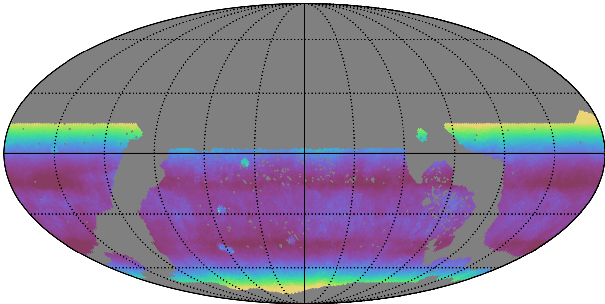
too_10_4v3.4_10yrs WFD i band: Median airmass
