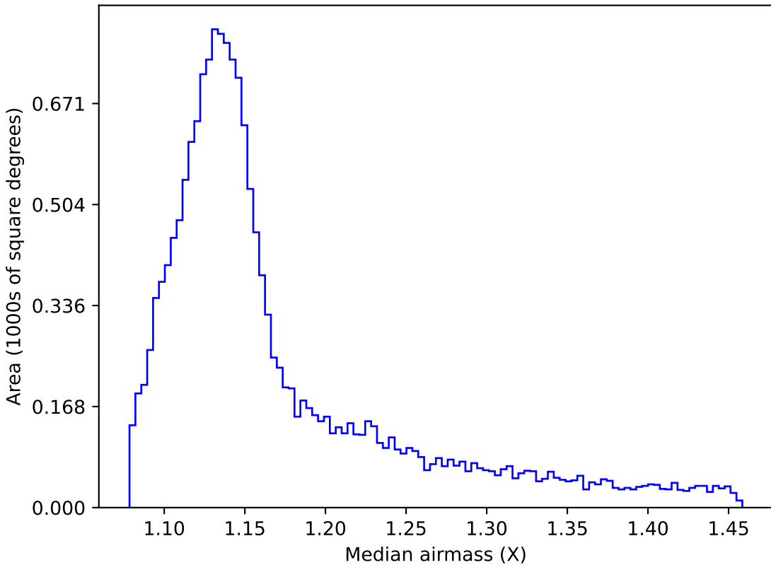
too_10_4v3.4_10yrs WFD i band: Median airmass
