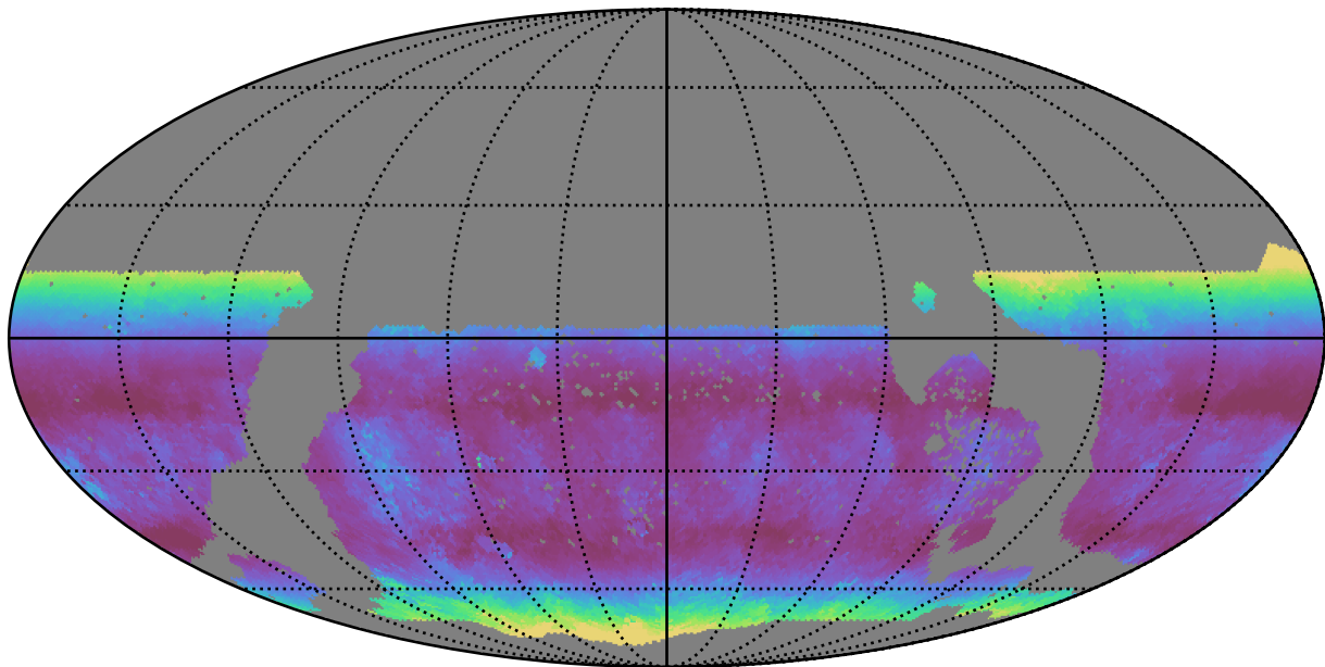
too_10_4v3.4_10yrs WFD g band: Median airmass
