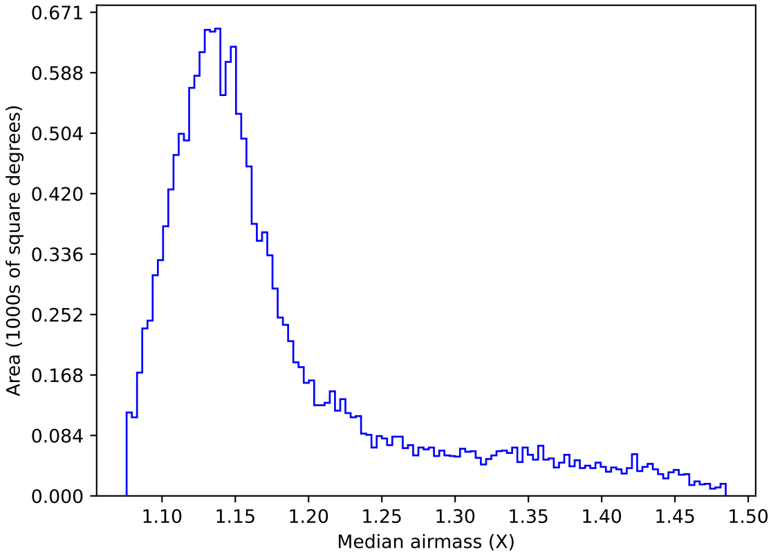
too_10_4v3.4_10yrs WFD g band: Median airmass
