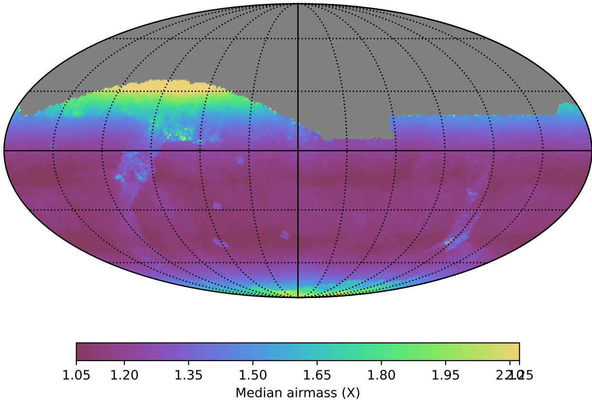
too_10_4v3.4_10yrs All sky z band: Median airmass
