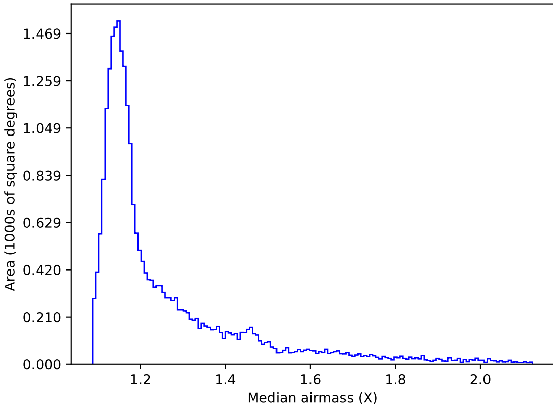
too_10_4v3.4_10yrs All sky z band: Median airmass
