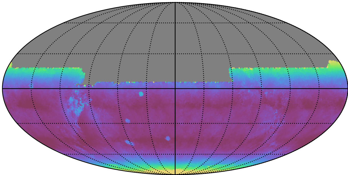
too_10_4v3.4_10yrs All sky y band: Median airmass
