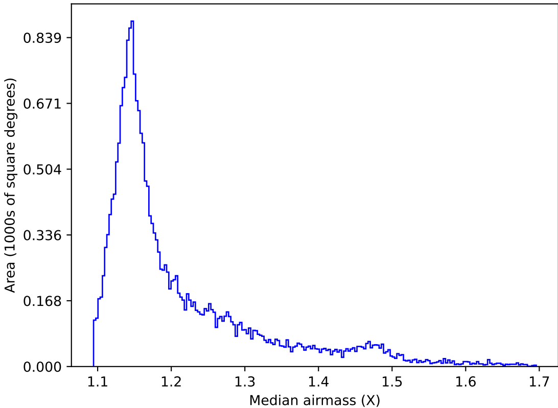
too_10_4v3.4_10yrs All sky y band: Median airmass
