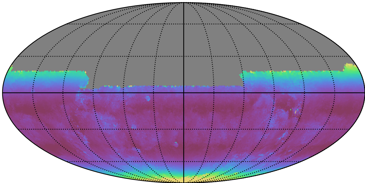
too_10_4v3.4_10yrs All sky u band: Median airmass
