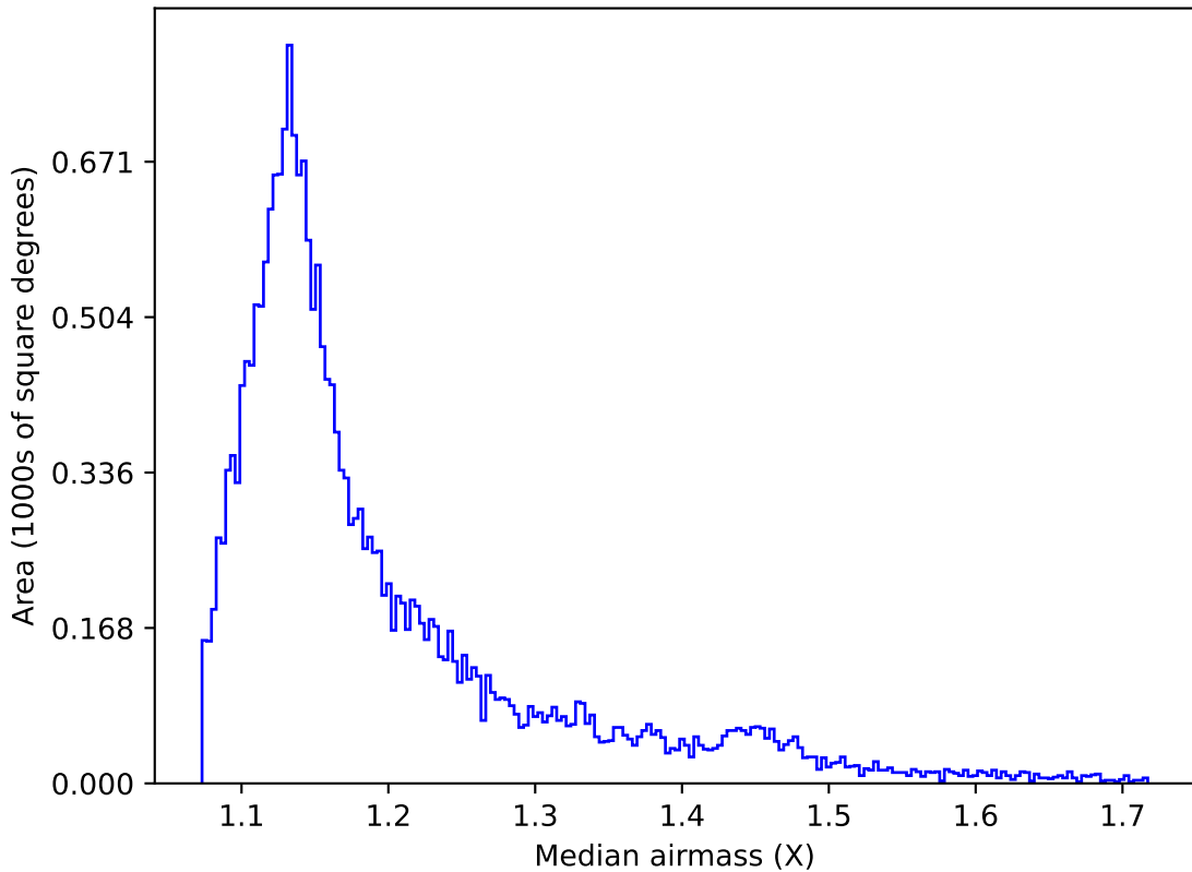
too_10_4v3.4_10yrs All sky u band: Median airmass
