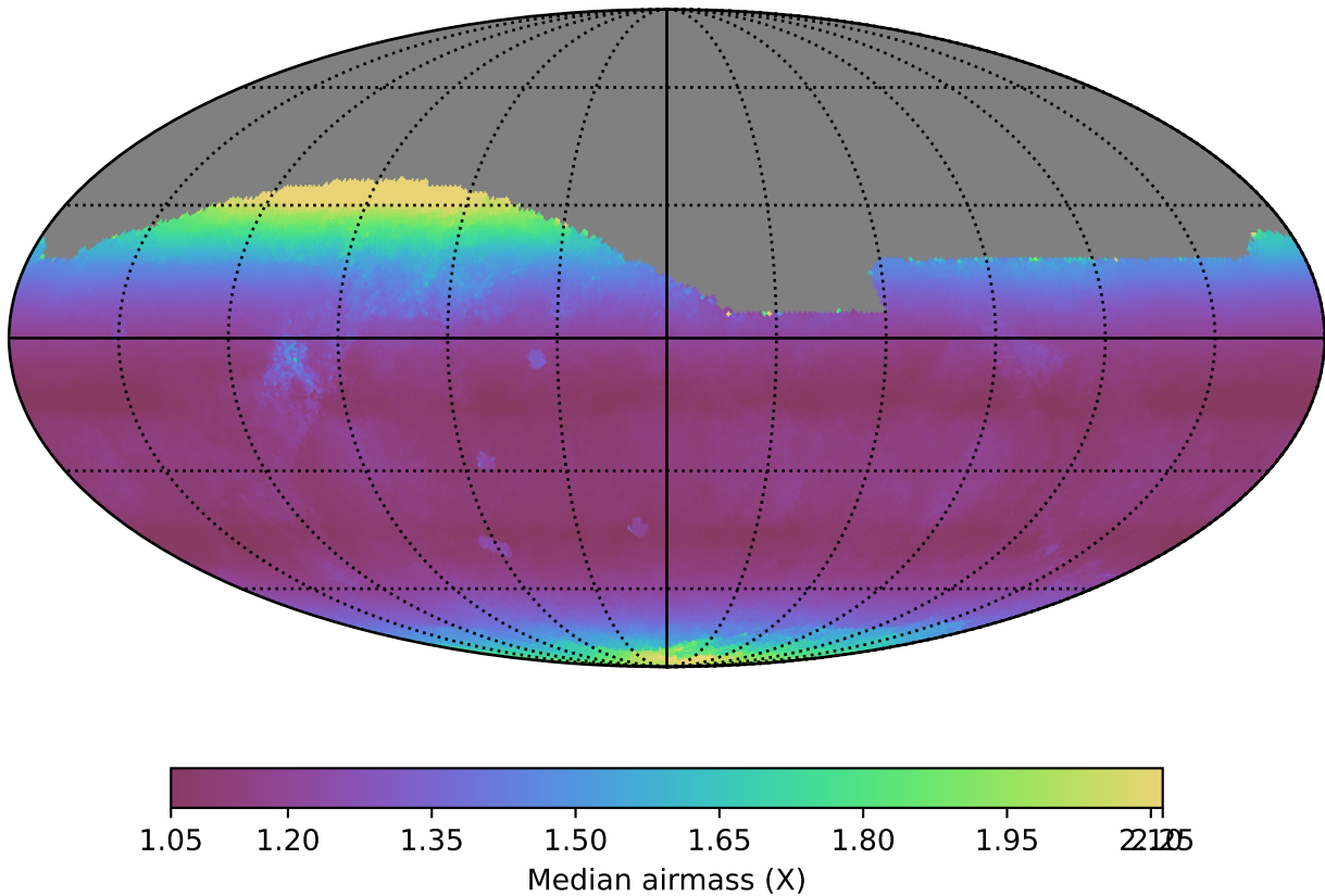
too_10_4v3.4_10yrs All sky r band: Median airmass
