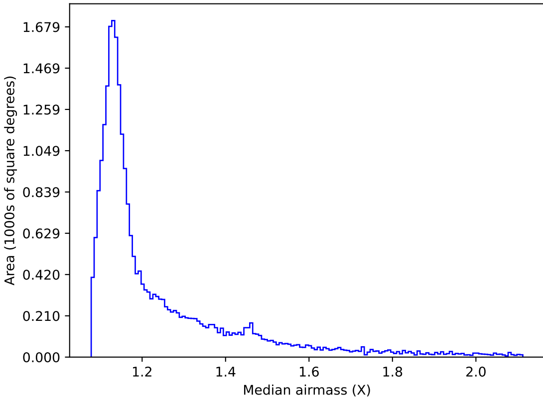
too_10_4v3.4_10yrs All sky r band: Median airmass
